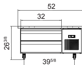
MGF8461GR
