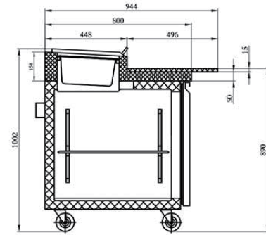
SECTION VIEW
