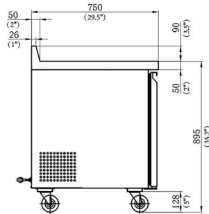
SECTION VIEW
