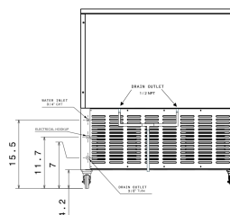
REAR UTILITY CONNECTIONS — Dimensions in inches
